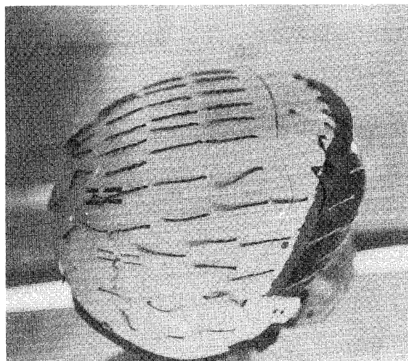
Fig. 12 Flow visualization, prototype mod 2, 0-deg angle of attack.
