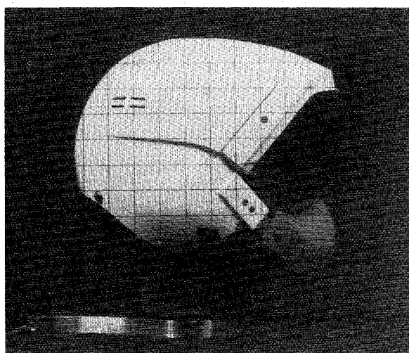
Fig. 4 Prototype helmet installed on cradle/headform assembly.
