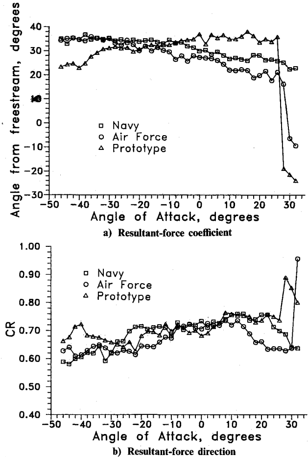
Fig. 8 Resultant-force magnitude and angle for baseline helmets.
