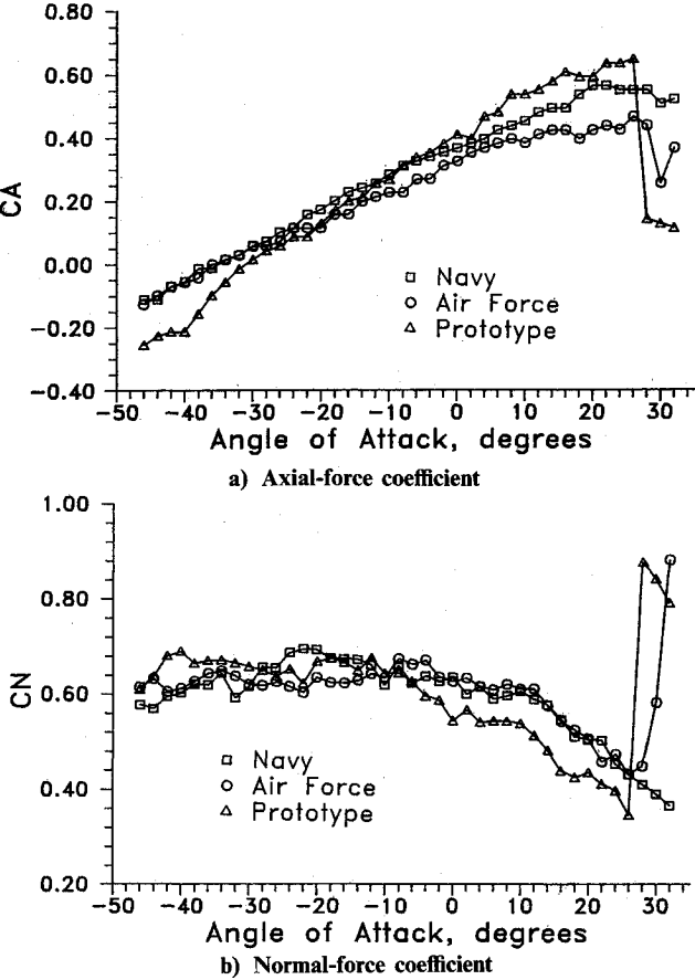
Fig. 7 Comparison of axial and normal forces for baseline helmets.
